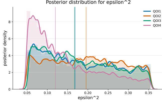
Figure 8: Posterior distribution over \epsilon^2
