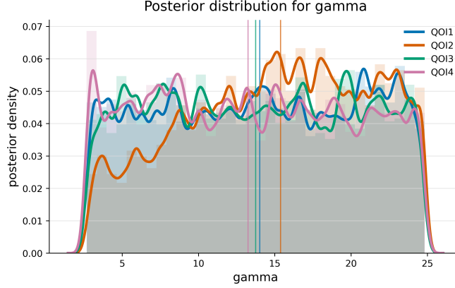
Figure 10: Posterior distribution over \gamma
