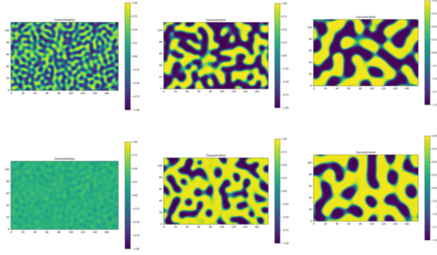
Figure 5: Snapshots of 2 simulations at different times. Column 1: Time = 10. Column 2: Time = 100. Column 3: Time = 1,000
