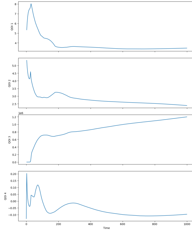
Figure 6: As the concentration field evolves, the QoIs are calculated for each snapshot. Convergence is desirable.
