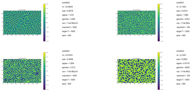
Figure 4: Cahn-Hilliard simulations
